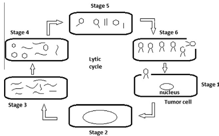
Fig. 1. The lytic cycle of oncolytic viruses.
