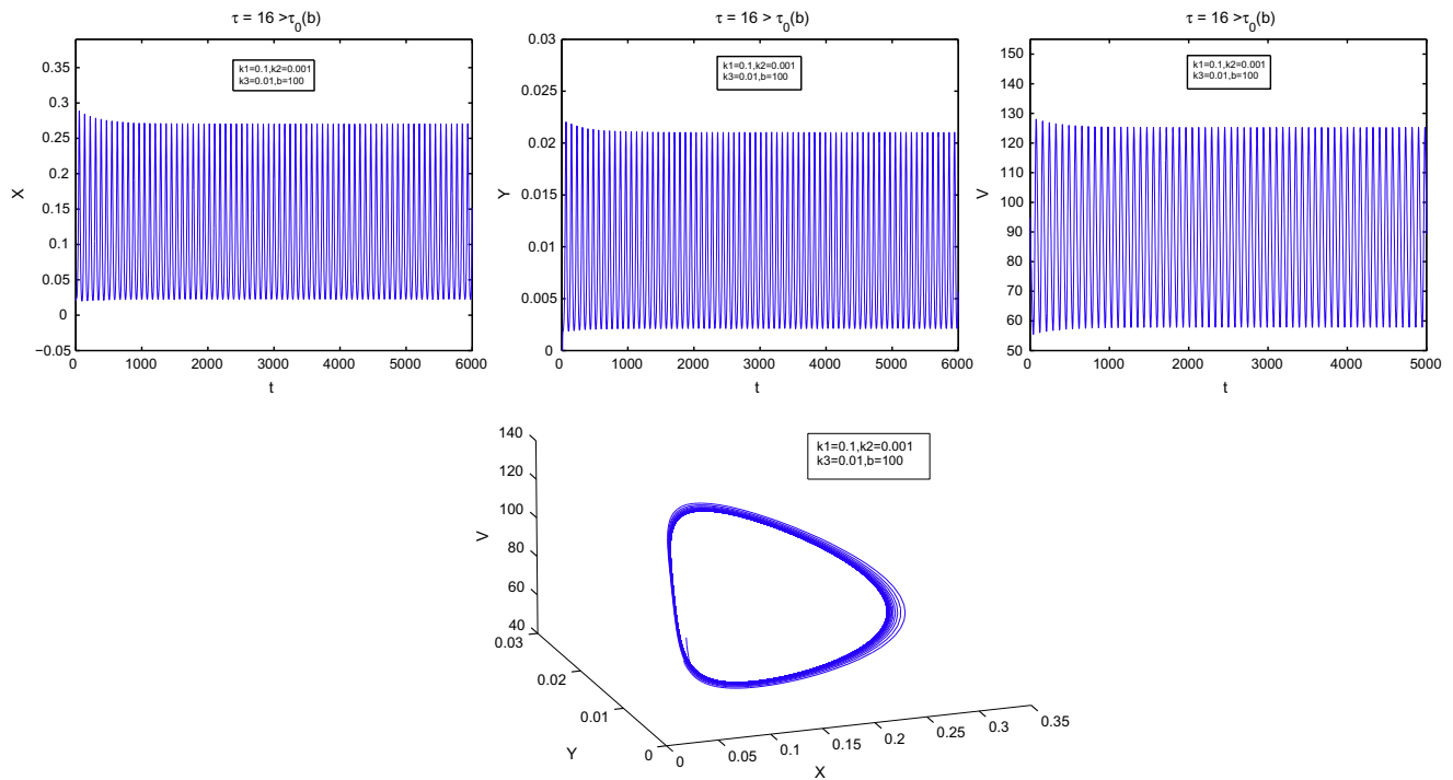
Fig. 5. Periodic solutions when \tau > \tau_0 .
