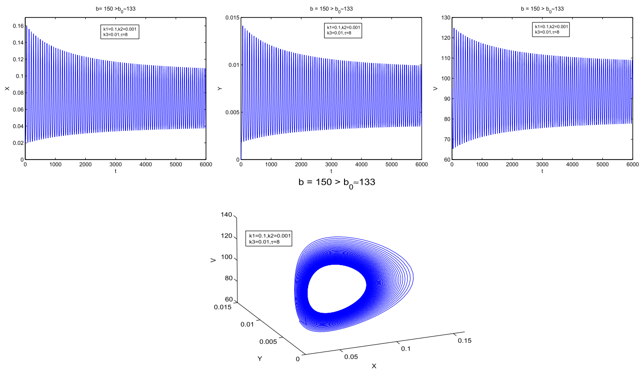
Fig. 7. Periodic solutions when b > b^* .
